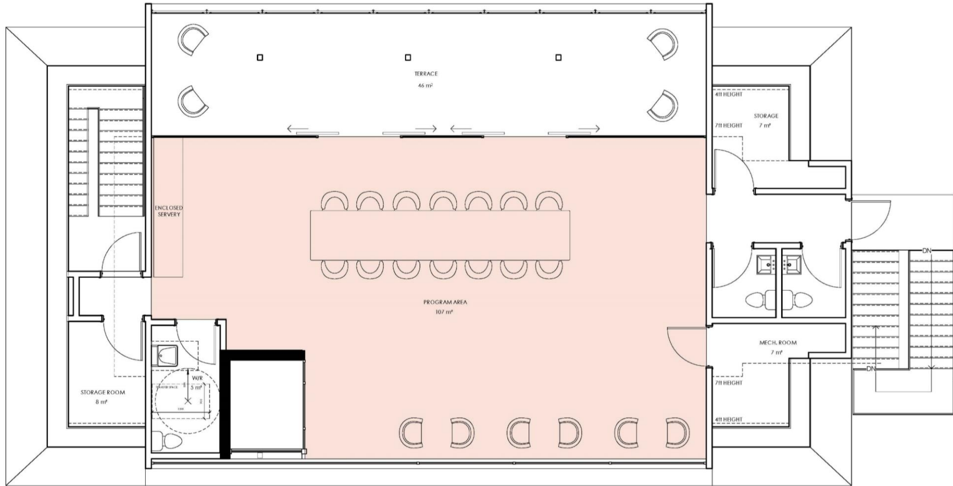
Level 4 | Open Space + Roof Terrace | Layout 1
